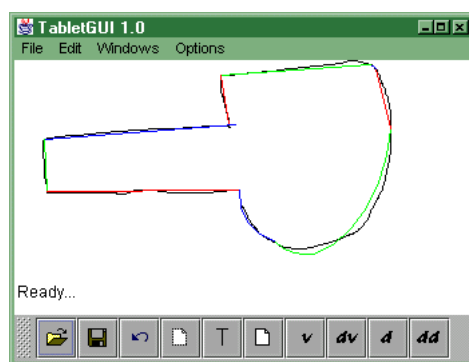
Figure 1: A stroke that contains both curves and straight lines (shown in black). The output generated by the recognizer system consists of Bézier curves and straight lines (shown in red, green, and blue).
