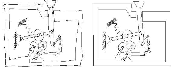
Figure 4. Input-output figures for the rough sketch of the direction reversal mechanism of a walkman.
